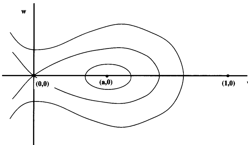
Level curves of E
