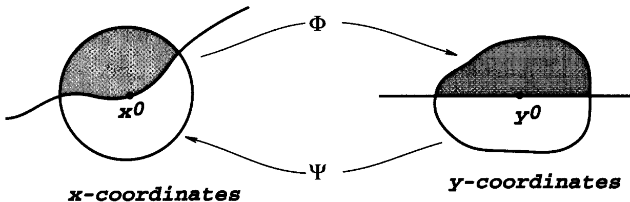
Straightening out the boundary
